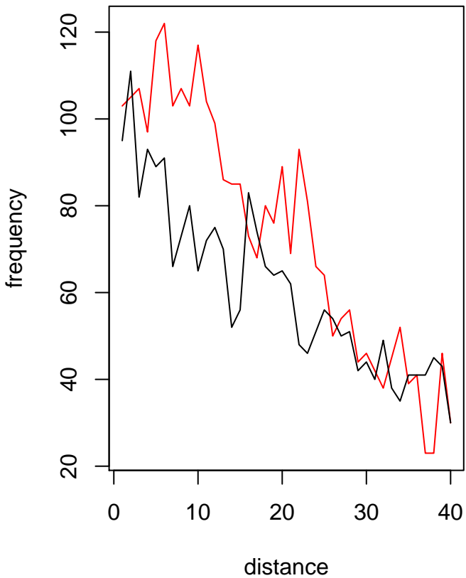
CTCF only
