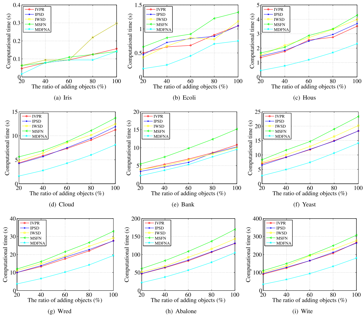
Fig. 1. The computational time of different algorithms versus different ratios of adding objects.
