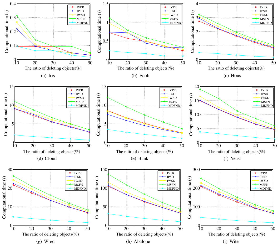
Fig. 2. The computational time of different algorithms versus different ratios of deleting objects.
