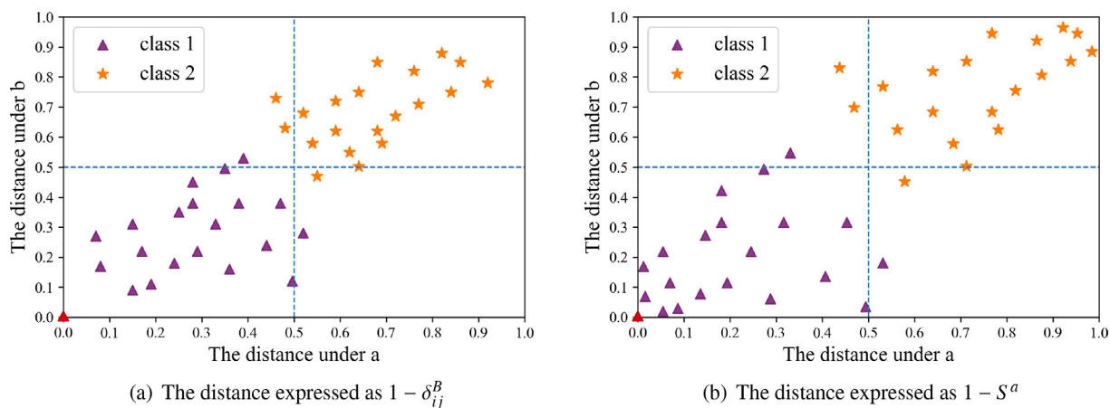
Fig. 2. Two types of distance between x^A and 40 samples.
