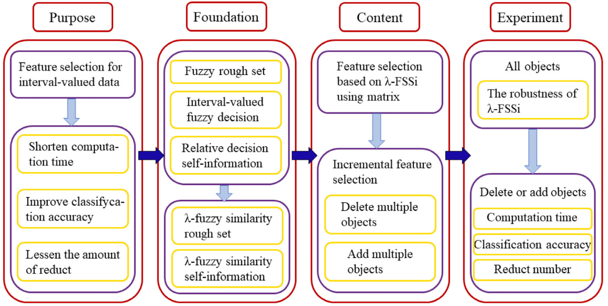
Fig. 1. The framework of our work.
