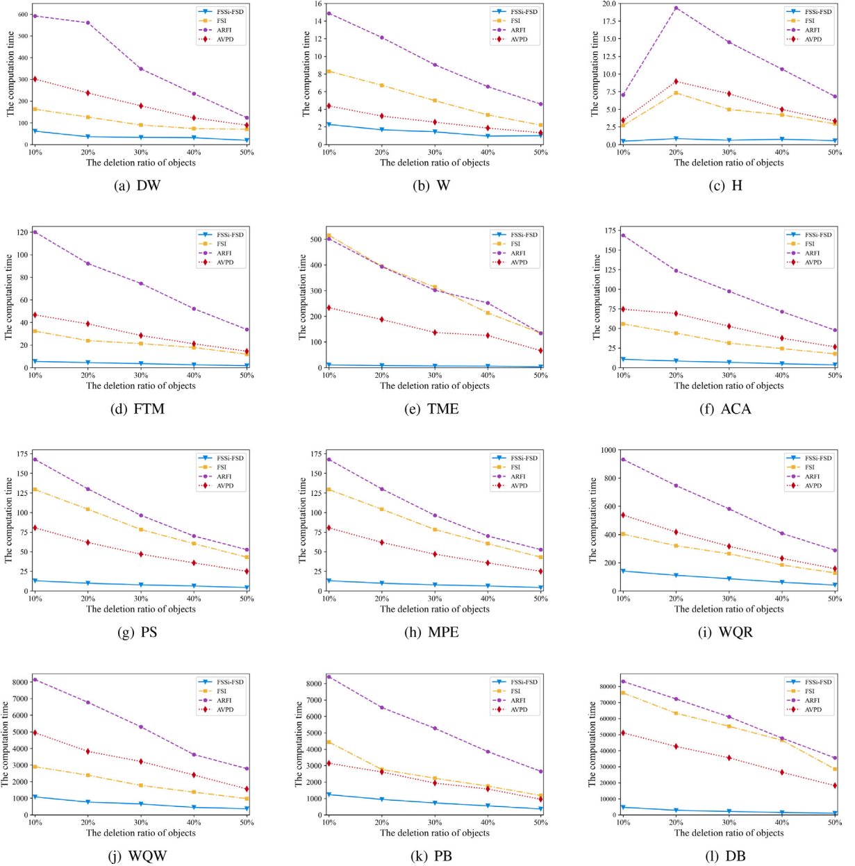
Fig. 6. The computation time among four algorithms with a certain ratio of deleting objects.
