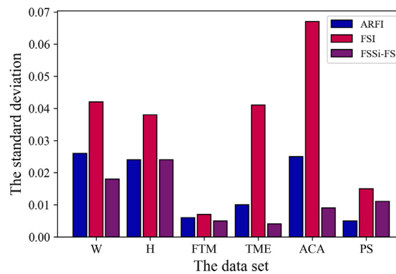
Fig. 5. The standard deviation of evaluation function about six data sets.
