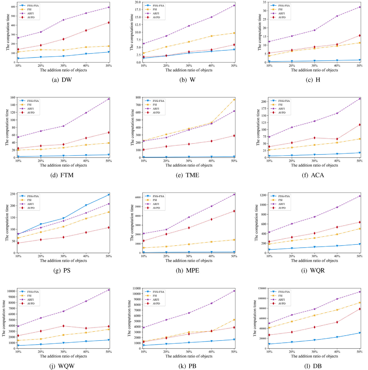
Fig. 7. The computation time among four algorithms with a certain ratio of adding objects.
