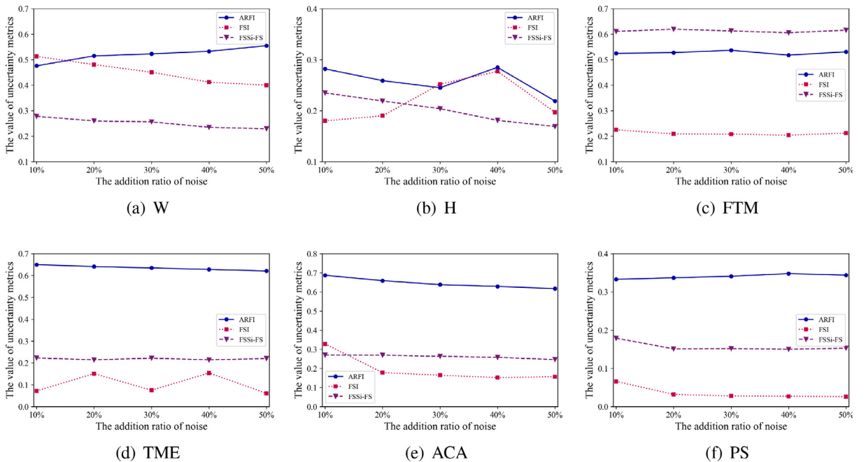
Fig. 4. The variation of evaluation function when adding a certain ratio of noise in IvFDIS.
