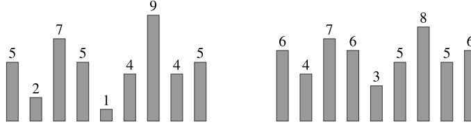
Fig. 2. Example of two order-isomorphic strings. Their codes are equal to (0, 0) (0, 1) (1, 0) (1, 1) (0, 2) (2, 4) (3, 0) (6, 6) (4, 4) .
