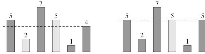
Fig. 1. To the left: w = 527514 . Here w_6 = 4 does not occur in w[..5] . We have \alpha(w) = 2 since w_2 = 2 the largest letter in w[..5] that is smaller than w_6 . Similarly, \beta(w) = 4 since w_4 = 5 is the rightmost occurrence of the smallest letter in w[..5] that is larger than w_6 . To the right: w = 527515 . Here w_6 = 5 occurs earlier in w . Therefore \alpha(w) = \beta(w) = 4 both indicate the position of the rightmost such occurrence.
