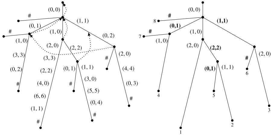
Fig. 4. The uncompact trie of \text{SufCodes}(w) for w = 12442551 (to the left) and its compacted version, the complete op-suffix-tree of w (to the right). The dotted arrows (left figure) show suffix links for branching nodes. One of them leads to an implicit node: \text{Locus}(255) = \text{Locus}(244) \rightsquigarrow \text{Locus}(25) = \text{Locus}(24) . This is because 2551 \not\approx 2442 but 255 \approx 244 and 551 \approx 442 . Boldface labels in the right figure are present also in the incomplete op-suffix-tree.
