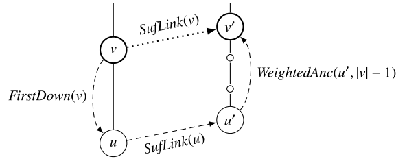
Fig. 6. Computation of \text{SufLink}(v) . Here u is explicit.
