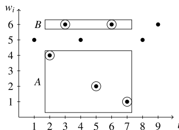
Fig. 8. Geometric illustration of the sequence w = 546526156 . The elements w_i are represented as points (i, w_i) . The computation of \text{LastCode}'(w[2..8]) = (3, 2) corresponds to counting points in rectangles A, B .
