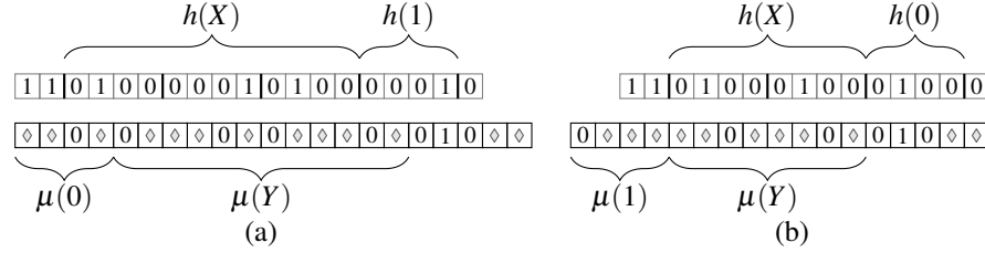
Figure 7: Illustration of Lemma 7: an occurrence of 11h(Xc)0 in \mu(c'Y)010\diamond\diamond for (a) Xc = 0101 , c'Y = 010 ; (b) Xc = 000 , c'Y = 100 . In general, 11h(Xc)0 is a prefix of \mu(c'Y)010\diamond\diamond if c = 1 and c' = 0 , and a suffix — if c = 0 and c' = 1 .
