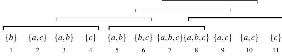
Figure 2: An indeterminate string of length 11 with a cover bcac . All occurrences of the cover are marked; the smallest covering set is \mathcal{C} = \{1, 5, 8\} (marked in bold).
