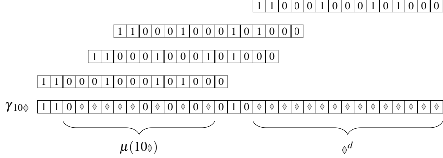
Figure 8: A gadget \gamma_{\diamond 01} with occurrences of a pattern 11h(110)0 .
