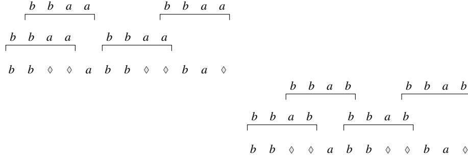
Figure 1: Partial word bb\diamond abb\diamond ba\diamond = bb\{a,b\}\{a,b\}abb\{a,b\}\{a,b\}ba\{a,b\} with its two shortest covers.
