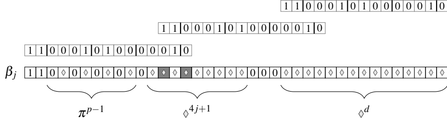
Figure 6: Sample gadget \beta_j for j = 2 and p = 3 with occurrences of a pattern 11h(101)0 . Positions d - 2 and d are marked in grey.
