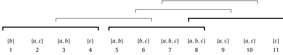
Fig. 2. An indeterminate string of length 11 with a cover bcac . All occurrences of the cover are marked; the smallest covering set is C = \{1, 5, 8\} (marked in bold).
