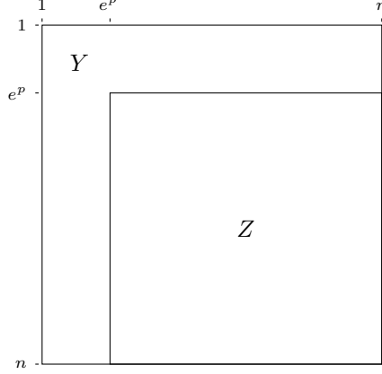
FIGURE 3.2. Matrix decomposition used in the proof of Theorem 3.1.
