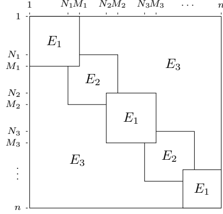
FIGURE 3.1. Illustration of the matrix decomposition used in the proof of Theorem 3.9. The figure is drawn for clarity on a log log scale.
