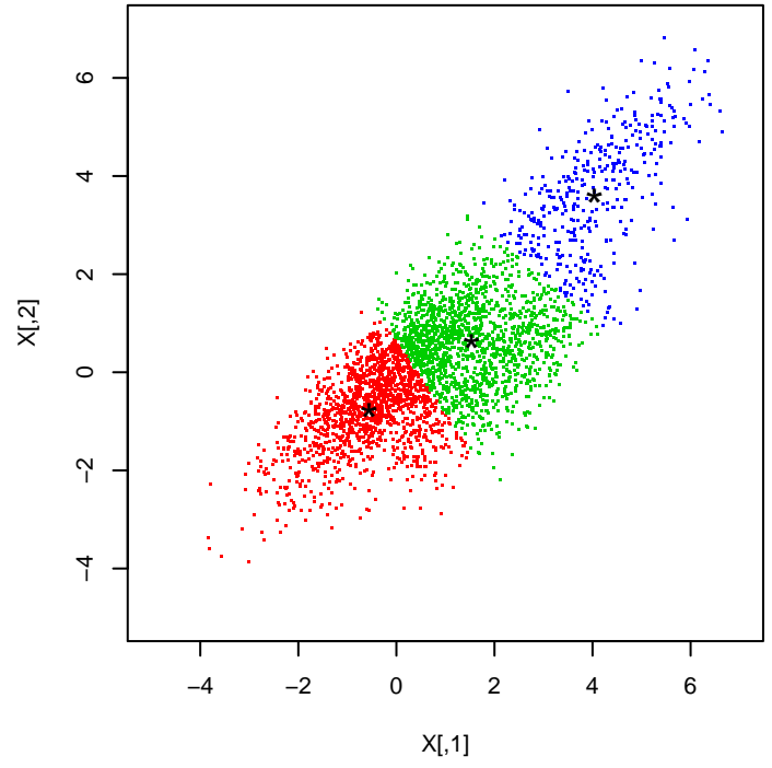
k-means
