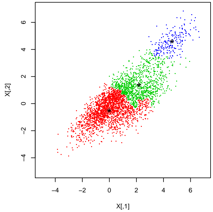
hclust
