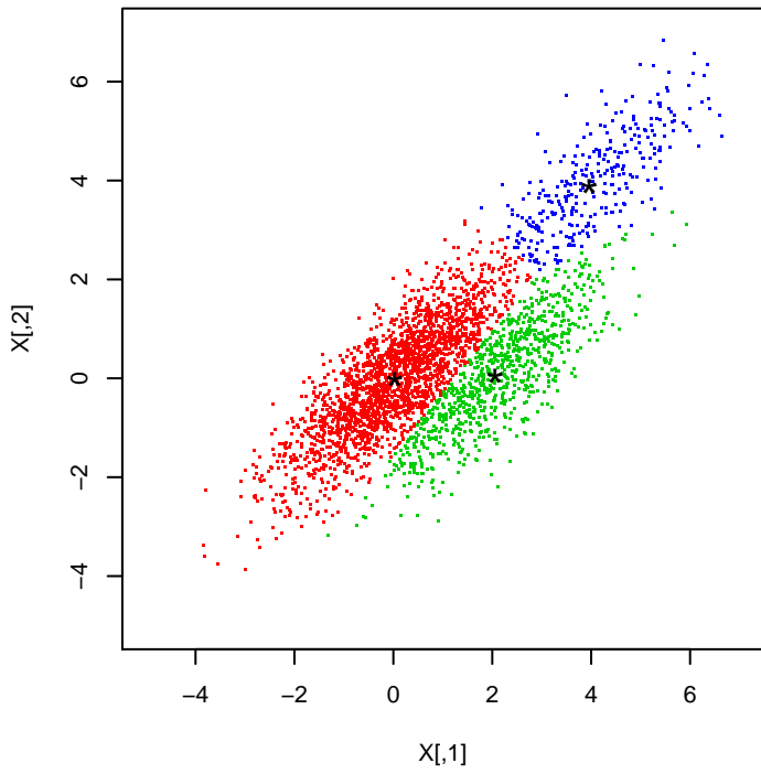
mclust
