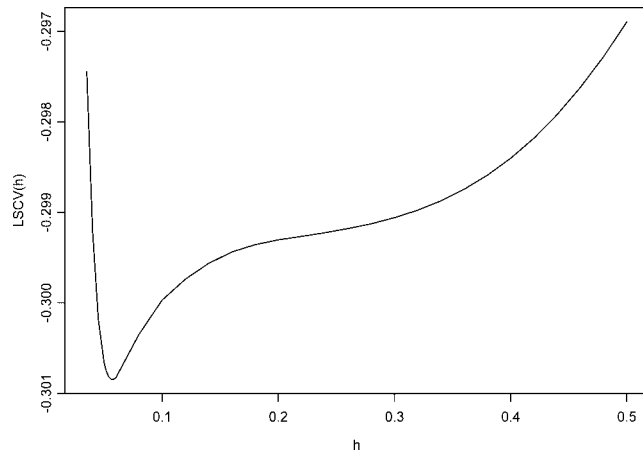
FIG. 3. Plot of the least squares cross-validation function LSCV(h) against h .
