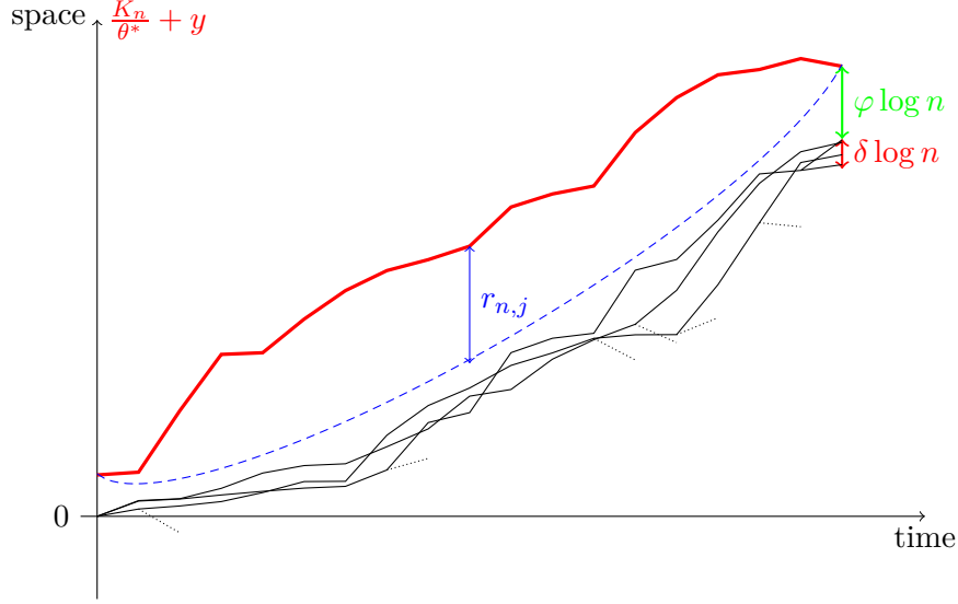
Figure 2: Some trajectories counted in X_n(\delta)
