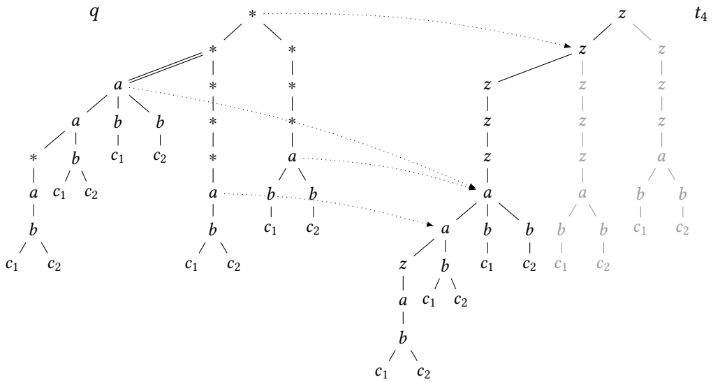
(d) How q can be matched in canonical tree model t_4 of p
