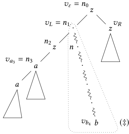
Fig. 20. Sketch of a tree t , as used in the proof of (C)
