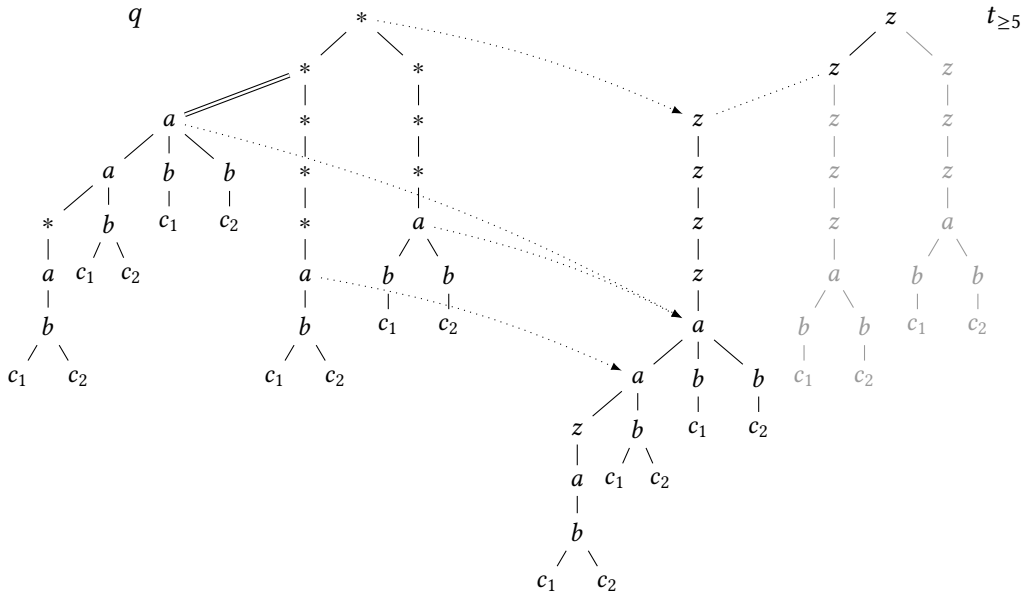
(e) How q can be matched in all other canonical tree models of p
