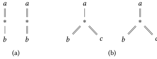
Fig. 12. Two examples of two equivalent minimal tree patterns
