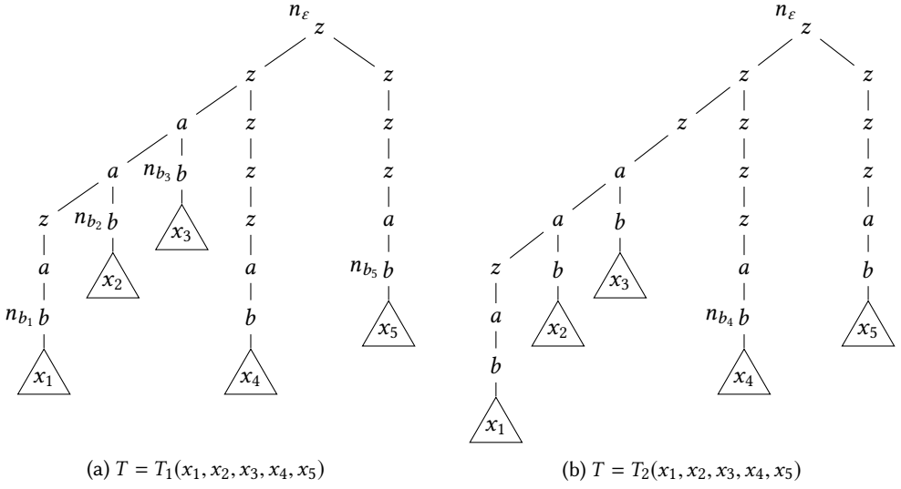
Fig. 17. Gadget for making canonical tree models for the proof of Lemma 7.11
