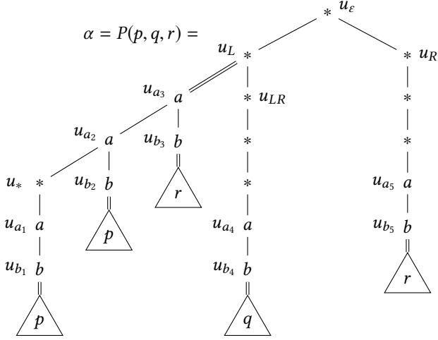
Fig. 16. The main gadget, instantiated with patterns p , q , and r , and annotated with node names for the proof of Lemma 6.3
