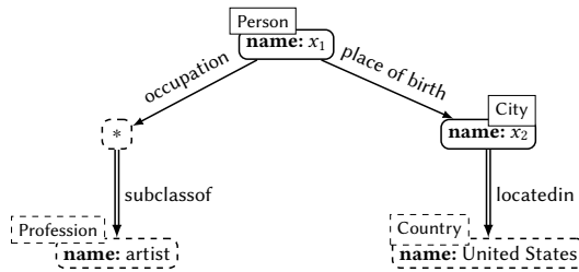
Fig. 2. A tree pattern finding the artists who were born in the United States. The query returns the person names and the cities where they were born. (Fully circled nodes are return nodes.)
