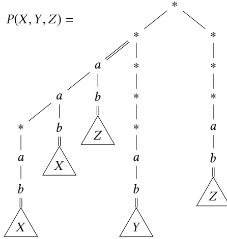
Fig. 13. Gadget for constructing tree patterns (Section 5.2 and Lemma 6.3)
