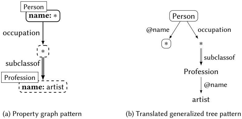
Fig. 6. Translating a subquery of Figure 2 to our simplified model
