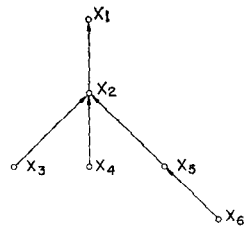
Fig. 1. Example of a dependence tree.
