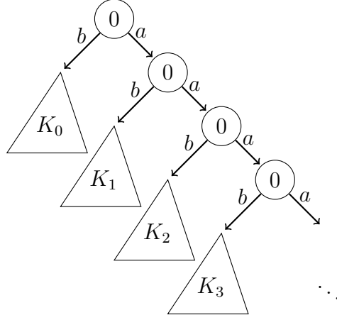
Figure 1: The coloring K obtained as a join of K_n 's. Applies to Facts 3 and 4.
