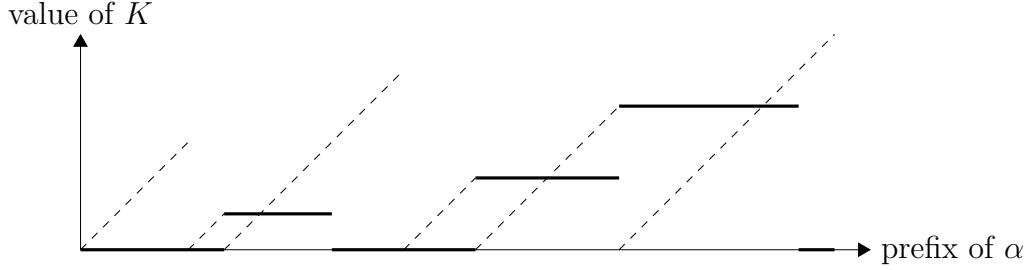
Figure 2: Values of K on prefixes of some \alpha \in A^\omega . Dashed line presents the number of trailing a 's in a given prefix of \alpha .
