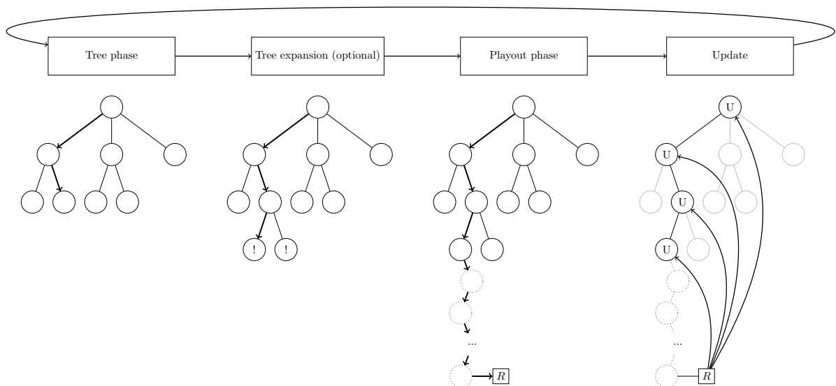
Figure 3.3: Four stages of every rollout.
