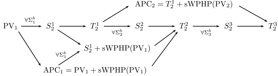
FIGURE 1. The prior-studied fragments of bounded arithmetic based on approximate counting. The arrows show the direction of inclusion, and the labels show conservativity. For instance, T_2^2 proves APC_1 and S_2^1 is \forall\Sigma_1^b -conservative over PV_1 . In addition to the inclusions shown, S_2^1 + \text{sWPHP}(PV_1) is a subtheory of APC_2 .
