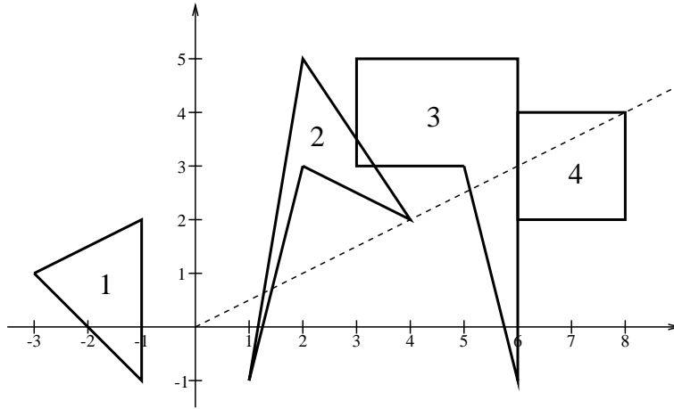
Figure 1: Semi-line for the sample input data.
