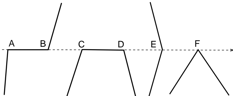
Figure 2: A collection of nasty cases to consider
