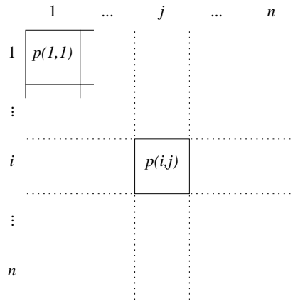
Figure 3: Coordinates of the fields
