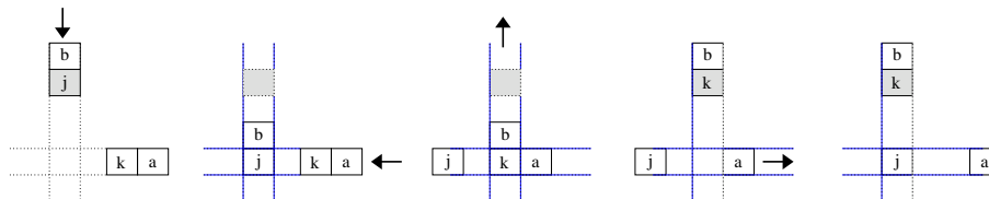
Figure 5: Four shifts to move the piece no. k to the proper (gray) field, provided that it was in improper row and column.
