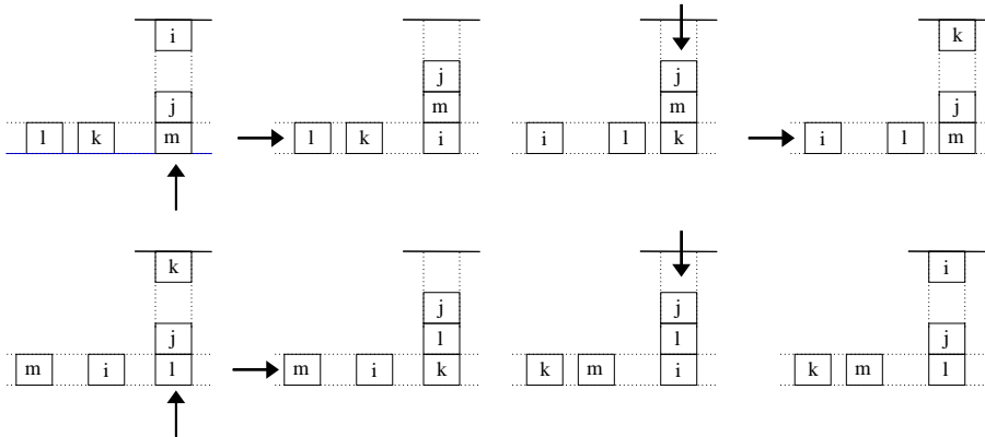
Figure 6: Rearranging the last row: k moves to l 's place, l to m 's place and m to k 's place.
