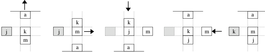
Figure 4: Four shifts to move the piece k to the proper (gray) field, provided that it was already in the proper row.
