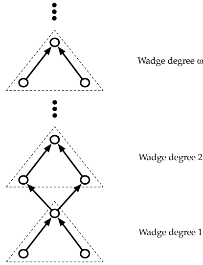
Figure 1: The Wadge hierarchy: circles represent Wadge-equivalence classes and arrows stand for the strict Wadge reduction between those. The non-self dual sets and the self dual ones located just one level above share the same Wadge degree.
