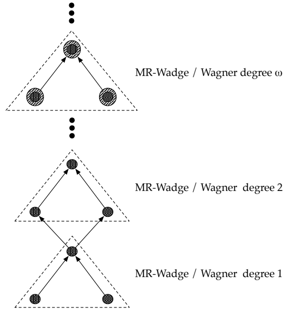
Figure 2: The MR-Wadge and the Wagner hierarchy. On finite levels the classes coincide; above, MR-Wadge classes properly extend corresponding Wagner classes.
