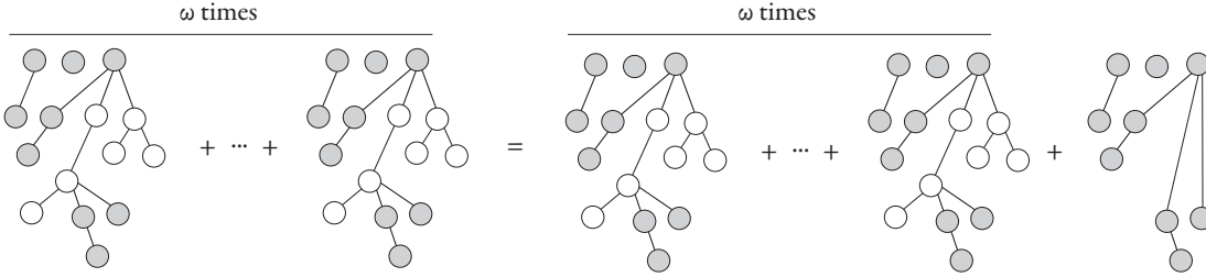
Figure 3: The identity \omega(\mathbf{vuh}) = \omega(\mathbf{vuh}) + \mathbf{vh} , with the white nodes belonging to \mathbf{u} .
