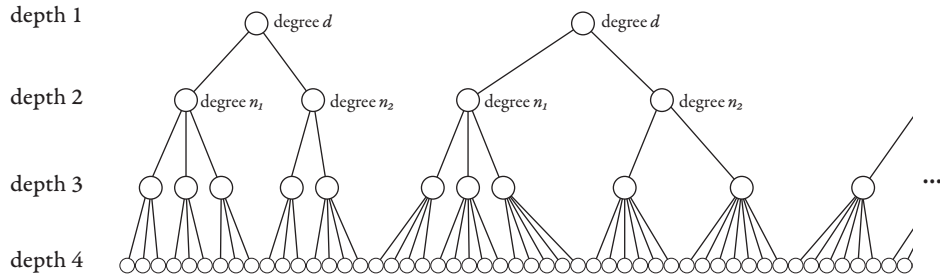
Figure 2: A sequence of trees as in Lemma 3.2. Here d = 2 , n_1 = 3 , and n_2 = 2 .
