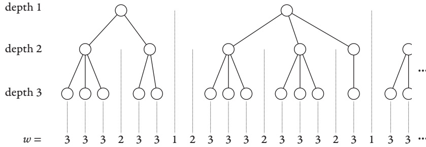
Figure 1: An example of \text{tree}(w) for n = 3 . Formally speaking, the the leaves of \text{tree}(w) are positions with label n , while the tree structure is defined by the following rule. Two leaves which correspond to positions x and y with label n have a common ancestor at depth i if and only if there is no position between x and y which has label in \{1, \dots, i\} . In particular, if between x and y there is a position with label 1, then x and y are in different trees of the sequence. Note that the mapping w \mapsto \text{tree}(w) is not one-to-one, e.g. in the picture, the first 2 just after the first 1 could be removed from w without affecting \text{tree}(w) .
