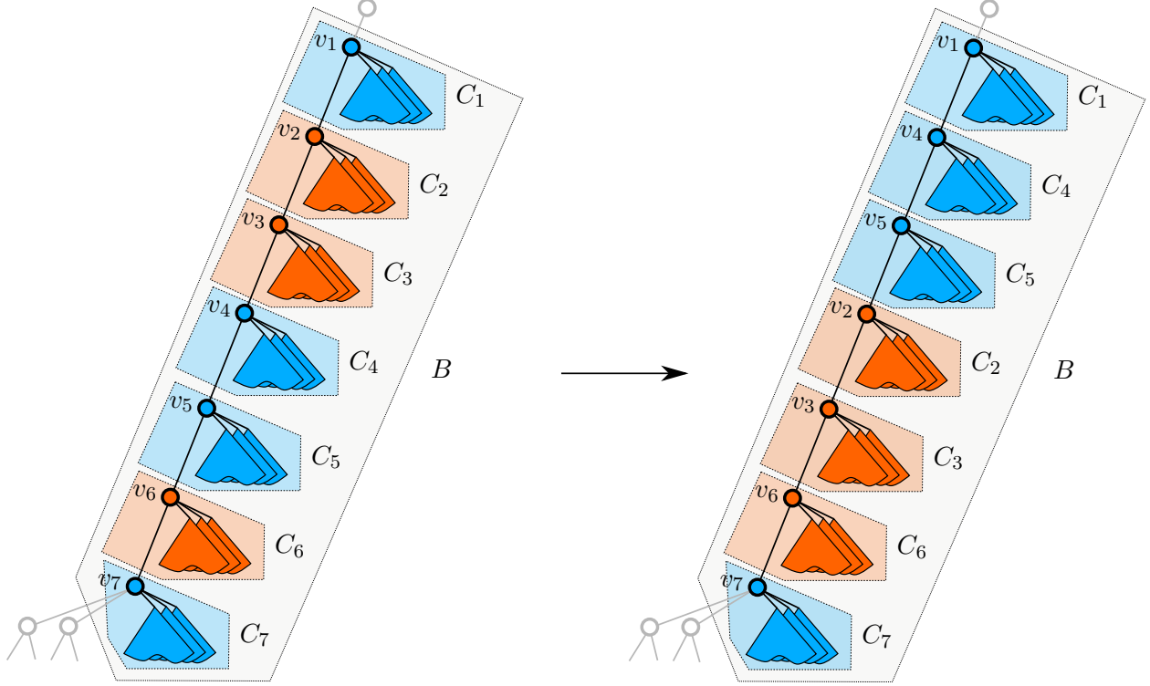
Figure 3: Reorganization of an example context B with 7 vertices on the spine. The context before the reorganization is on the left panel, after is on the right. The applied permutation is \pi = (1, 4, 5, 2, 3, 6) , and it leaves only two monochromatic blocks in h' . Note that the last context C_7 does not participate in the reorganization and stays on its place.
