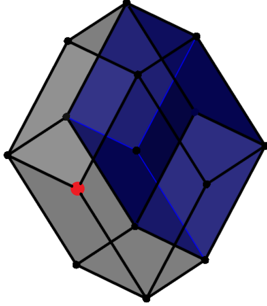
FIGURE 2. Newton polytopes of Example 6.7
