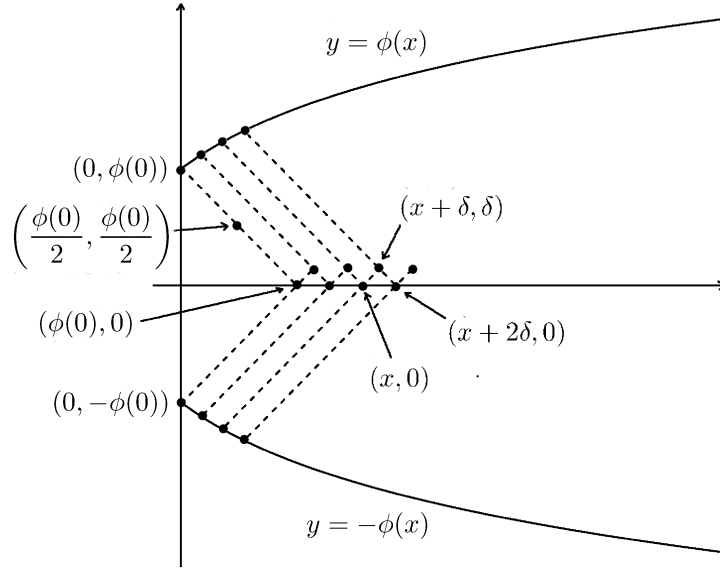
FIGURE 1. The structure of the extremal examples. The dots \bullet indicate the possible locations of the pair (f, \varphi) .
