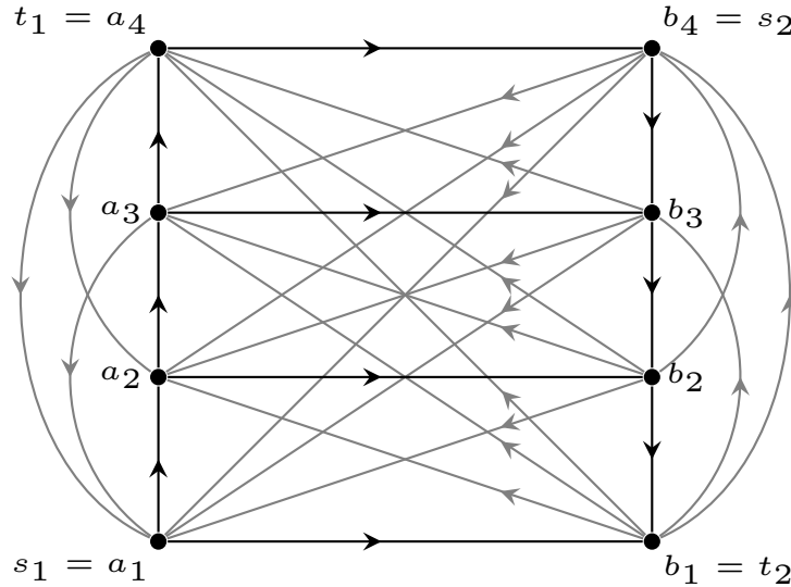
Figure 7.2: Tournament T_4 .
