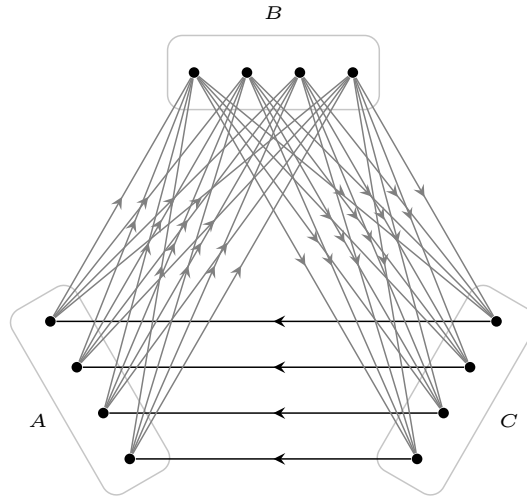
Figure 6.1: A 4-triple.
