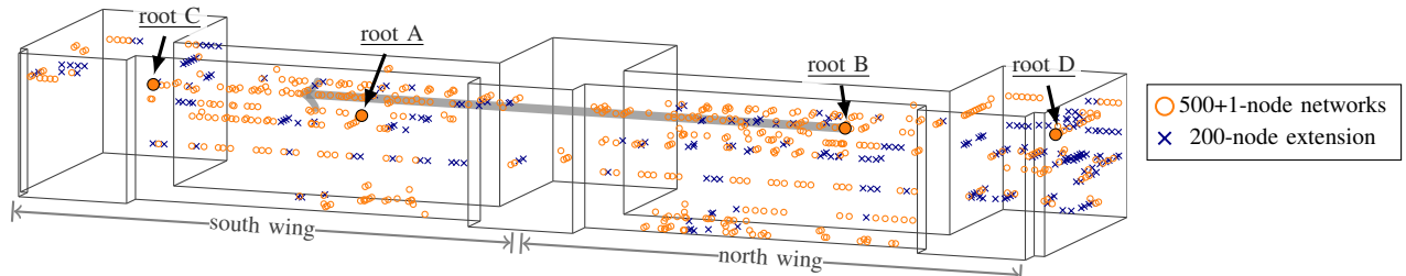
Fig. 1. Overview of the 500+1-node networks used in our evaluation, and the 200-node extension employed in Sect. III-F. Devices pointed by arrows are used as roots (one at a time). The gray arrow visualizes the link discussed in Sect. III-C (as if it were line-of-sight). The devices are deployed throughout the entire building for a total area of 3390m 2 with its north and south wings containing, respectively, 204+62 and 297+138 (base networks+extension) devices.
