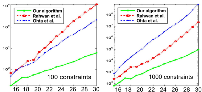
Figure 4: The time to solve the CSG problem given different algorithms, and different numbers of agents (log scale).
