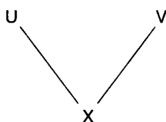
Figure 2. Orienting the edges.
