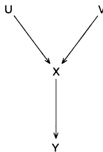
Figure 1. Directed acyclic graphs.
