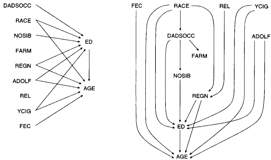
Figure 3. The left-hand panel shows the model reported by SGS (1993, 140). The right-hand panel shows the whole graph produced by the SGS search program TETRAD II. 14
